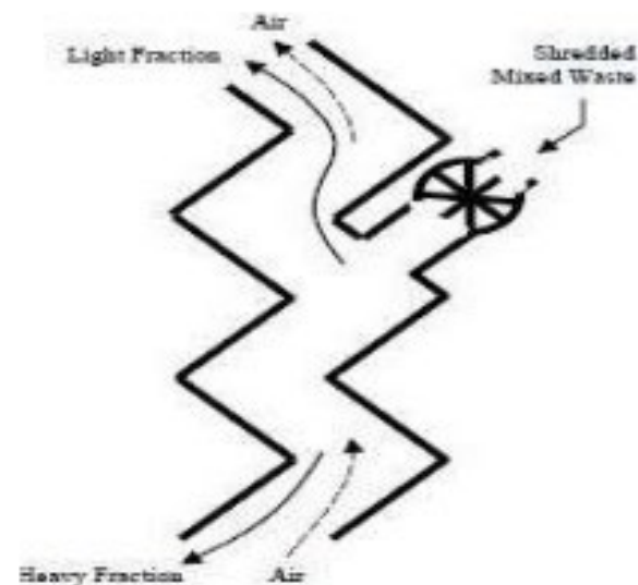
Types of vertical air classifiers
